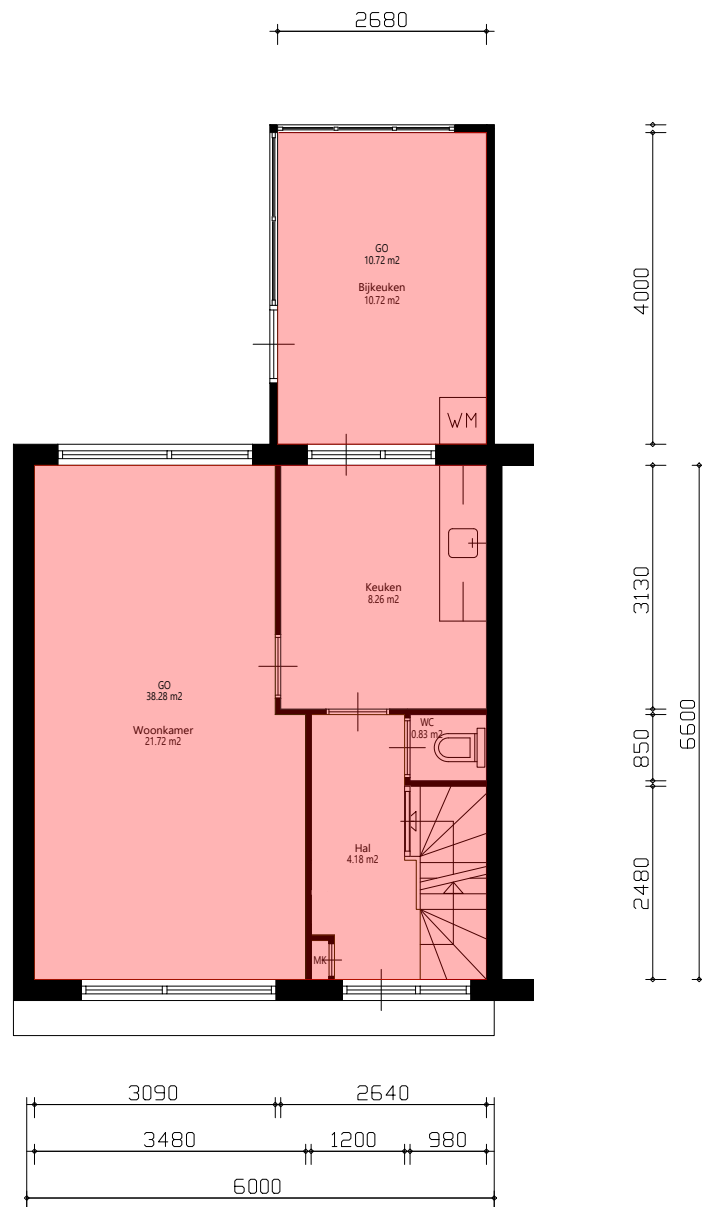
Begane_grond
